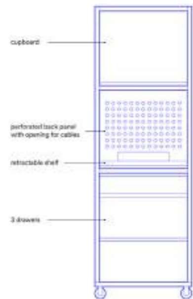
SINGLE UNIT 06
