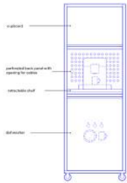
SINGLE UNIT 01
